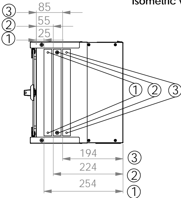
Isometric views
