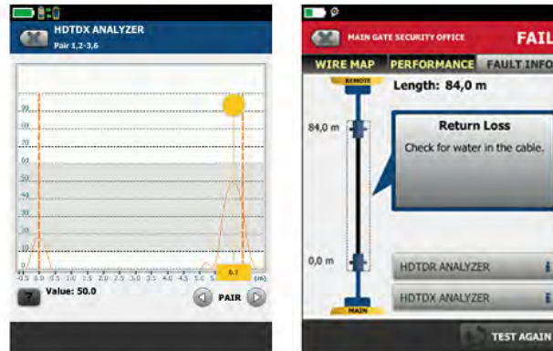
High Definition Time Domain Cross talk (HTDIX) shows the far end connection is clearly the issue
