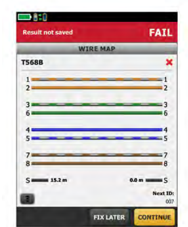
Wiremap – shows distance to fault, break and short
