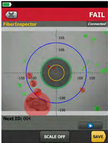
FiberInspector probe
